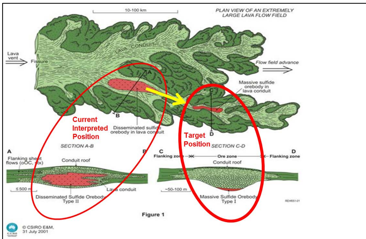
Figure 2: Schematic diagram of the Kambalda "Cabbage Leaf" Model showing the geological position of the mineralisation drilled to date at Talc Lake and the downstream target zone where the formation of massive Nickel Sulphide typically occurs.
