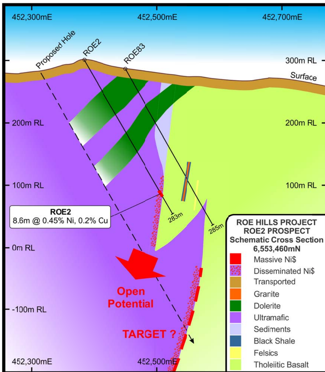
Figure 5: ROE2 Schematic Cross Section on 6,553,460mN
