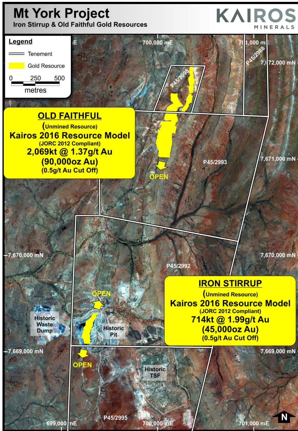
Figure 2 – Mt. York Iron Stirrup & Old Faithful plan view of 2016 Gold deposit resource models
