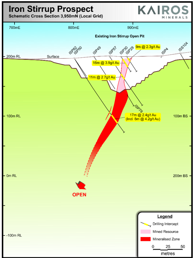
Figure 4 - Schematic Cross-Sections Showing the Iron Stirrup Deposit
