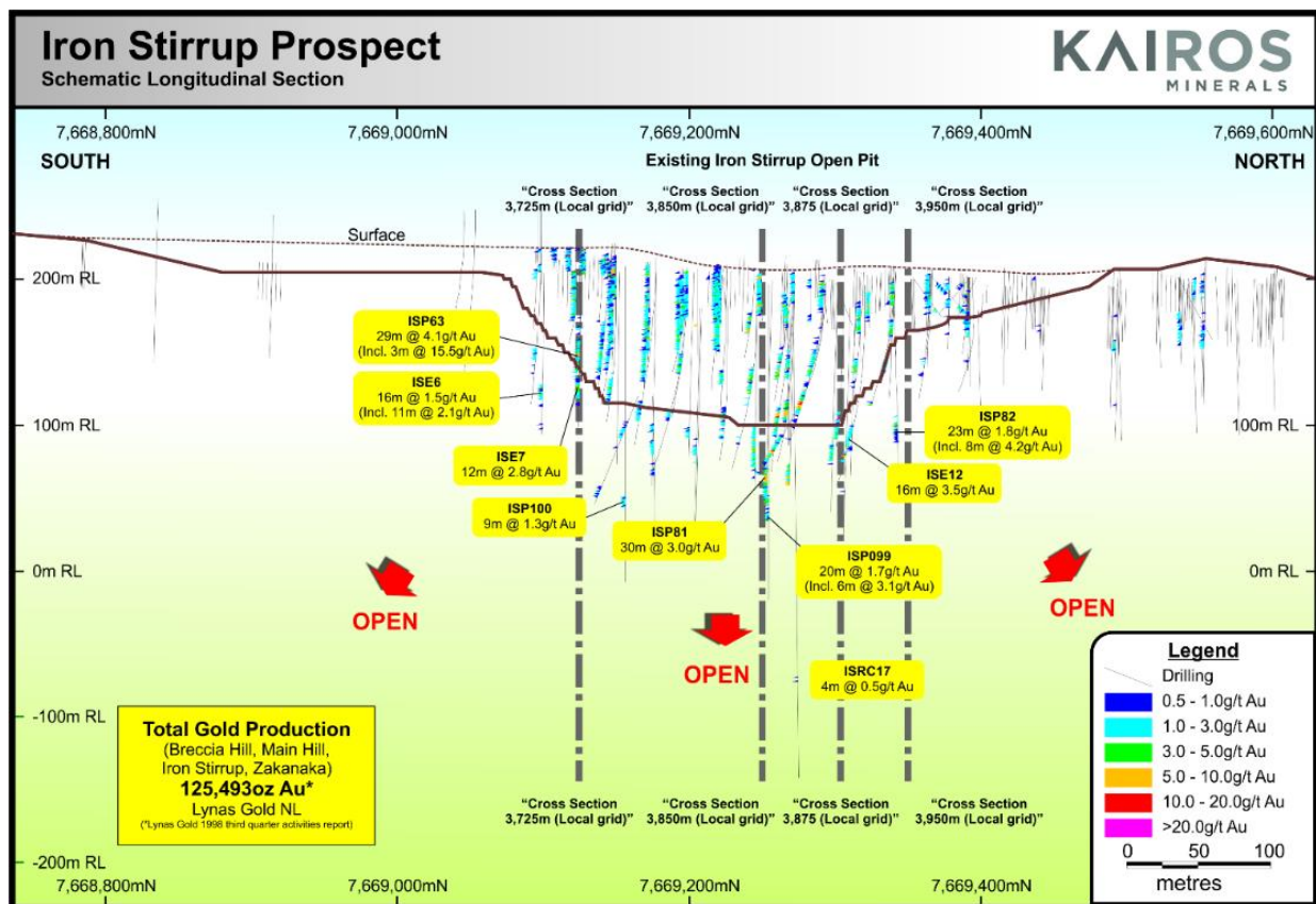
Figure 3 – Schematic Long Section of the Iron Stirrup Deposit
