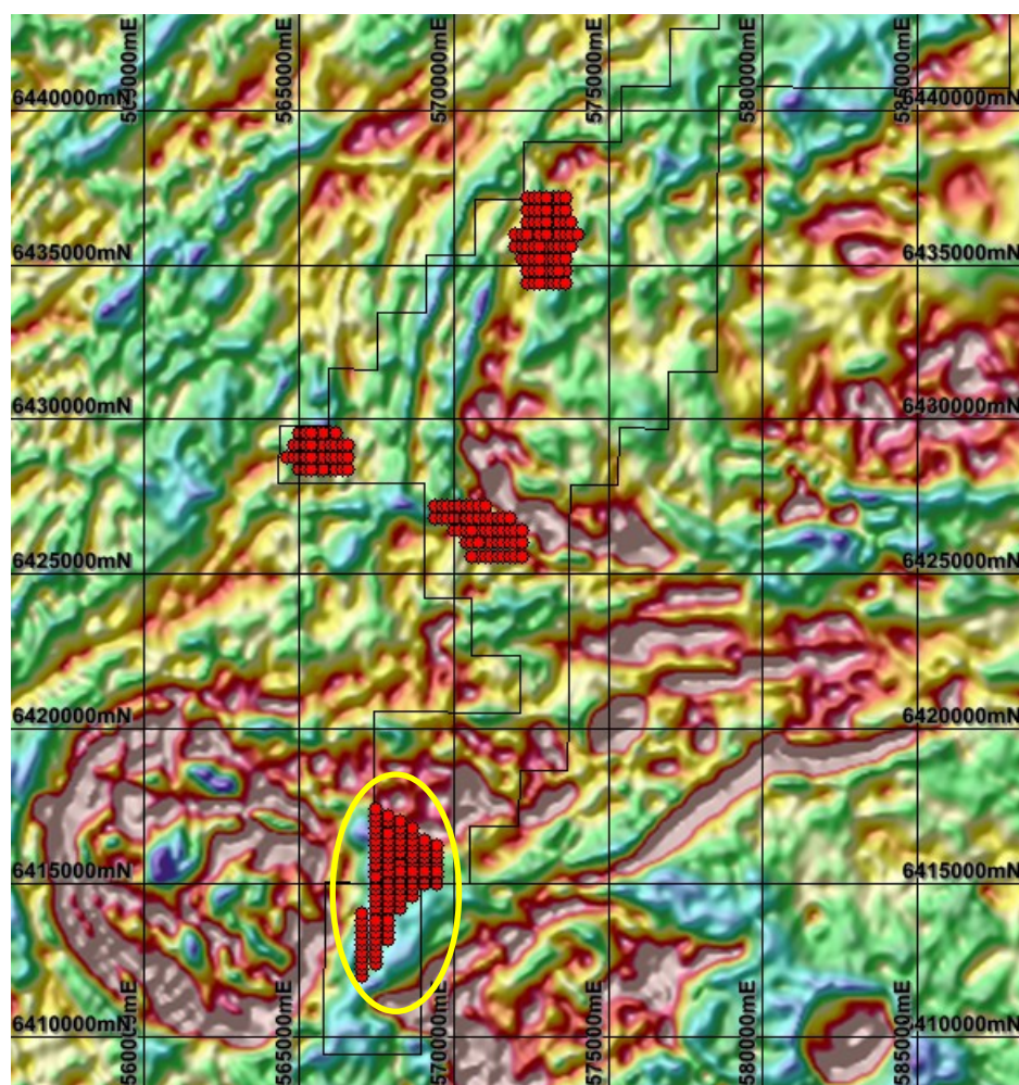
Figure 2. Aeromagnetic image of the Fraser Range geology showing all MLEM survey target zones. The yellow circle indicates the location of the Stage 1 target.
