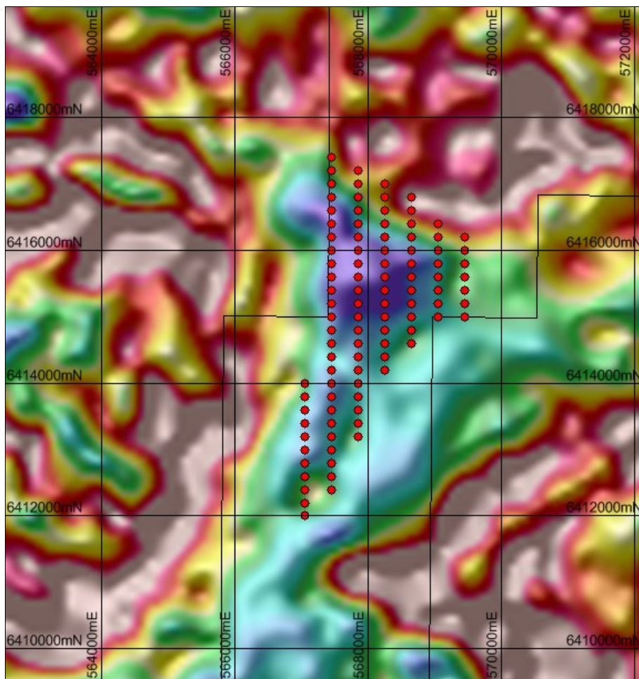
Figure 1. Stage 1 MLEM survey locations over priority aeromagnetic target zone.
